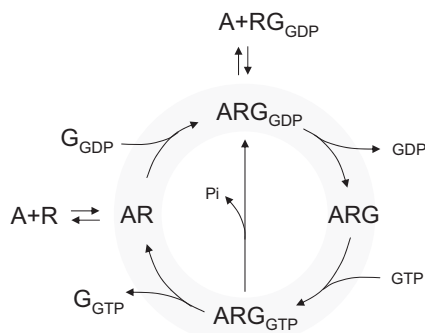
Scheme 1. Graphical representation of agonist-mediated G protein activation.
