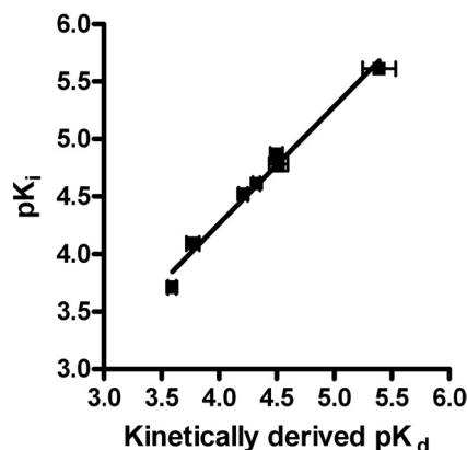
Fig. 4. Correlation between pK_i and kinetically derived pK_d for the seven test agonists. pK_i values were taken from [ ^3 H]NMS competition binding experiments at equilibrium (see Fig. 1). The values comprising the kinetically derived K_d ( k_{off}/k_{on} ) were taken from the experiments in Fig. 3. Data shown as mean S.E.M. ( n \geq 4 ).
