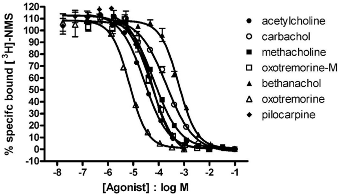
Fig. 1. Competition between [ 3 H]NMS and increasing concentrations of muscarinic agonists for muscarinic M 3 receptors in CHO cell membranes. Experiments were conducted in HBSS at 37°C. Because the total binding varied, data are shown as mean \pm range from a representative of four or more experiments performed in duplicate and plotted as the percentage of specific bound.
